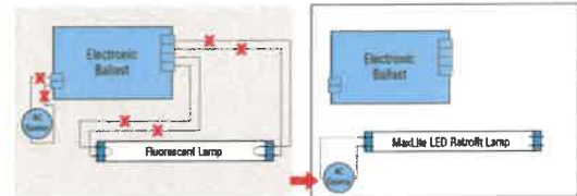
Figure 3. - Retrofit with One Lamp
