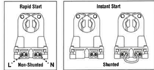
Figure 1. - Non-shunted & Shunted Lamp Holder
