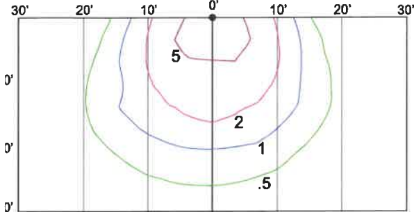
28W 3,640 LUMENS (SIZE 1 HOUSING) 10' MOUNTING HEIGHT
