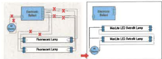
Figure 4. - Retrofit with Two Lamps
