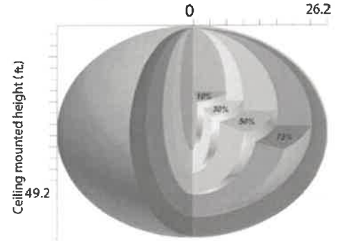
Model SAM6
