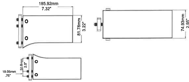
Straight Arm
