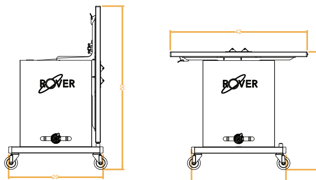
SIDE VIEWS
